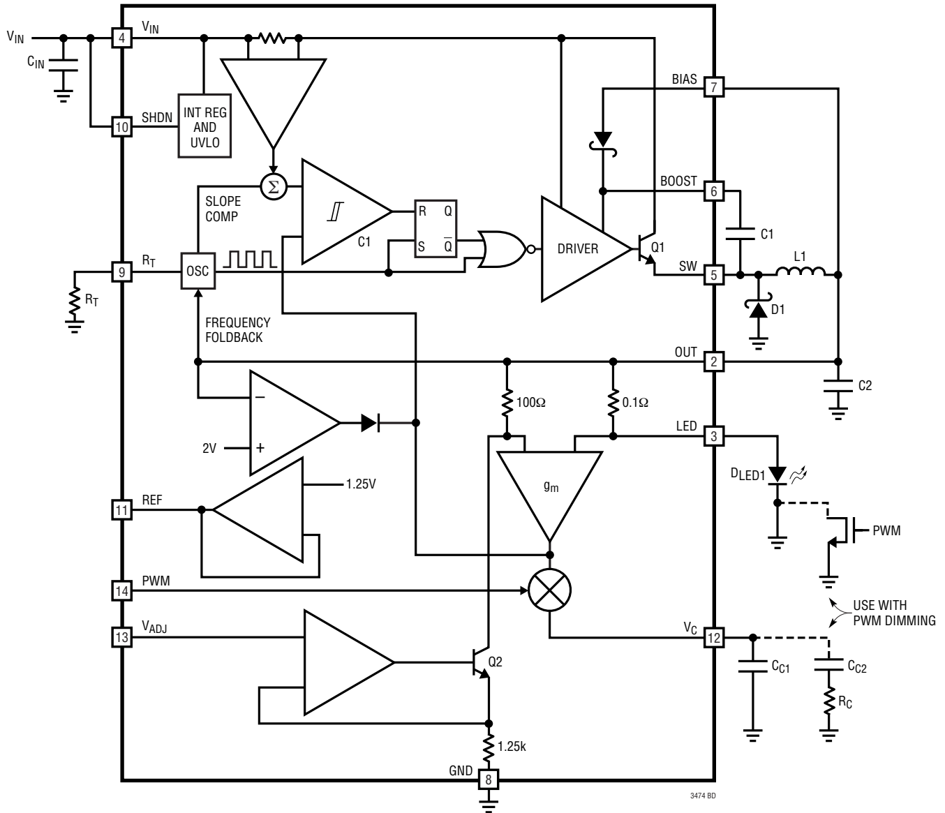
Figure 1. Block Diagram
