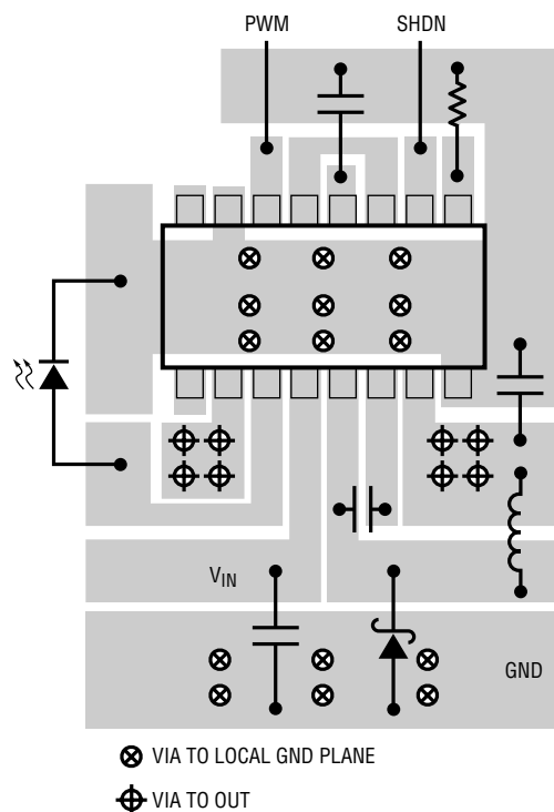
Figure 8. Recommended Component Placement
