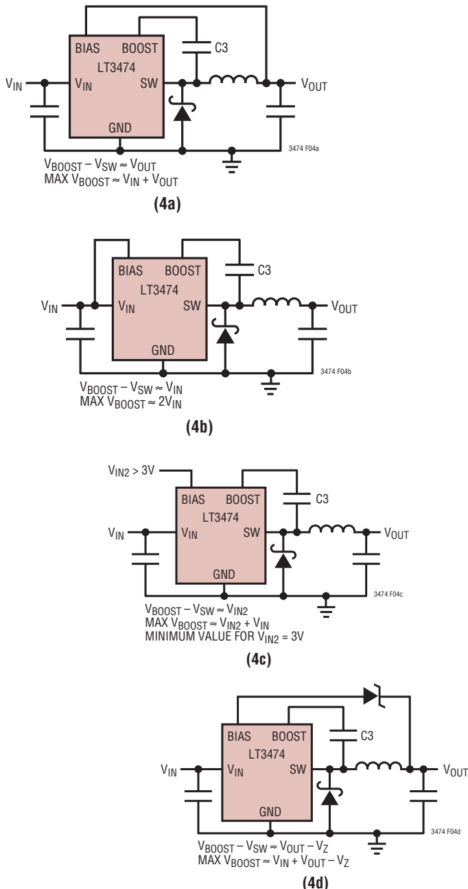
Figure 4. Generating the Boost Voltage
