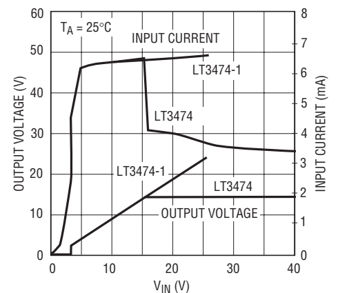
Open-Circuit Output Voltage and Input Current
